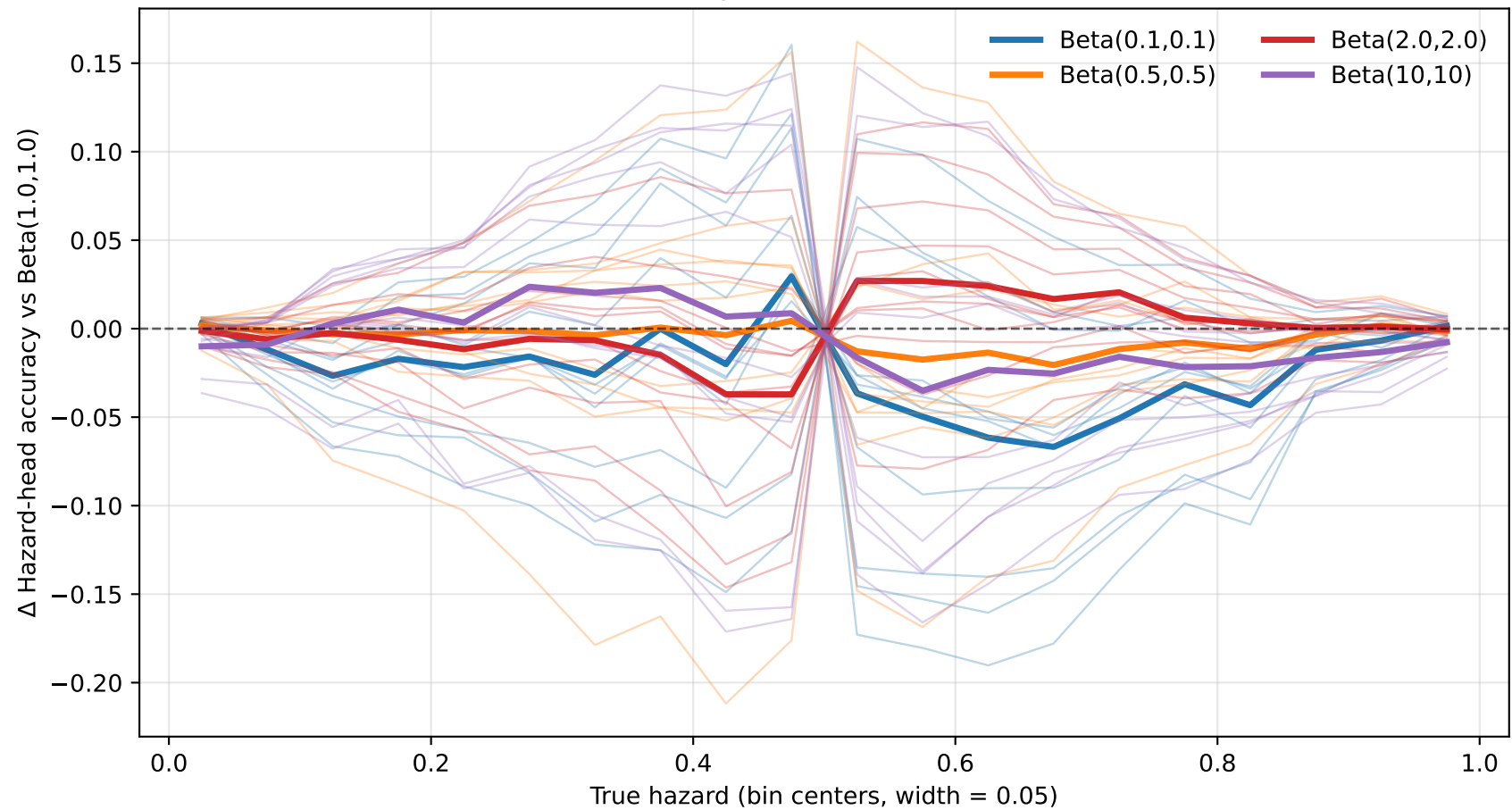
Hazard-head: accuracy difference relative to Beta(1.0,1.0)
